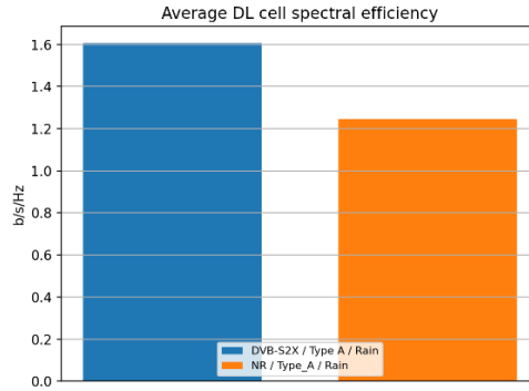
Figure 6: DL Average cell spectral efficiency
