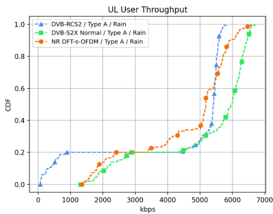
Figure 7: UL User throughput distribution
